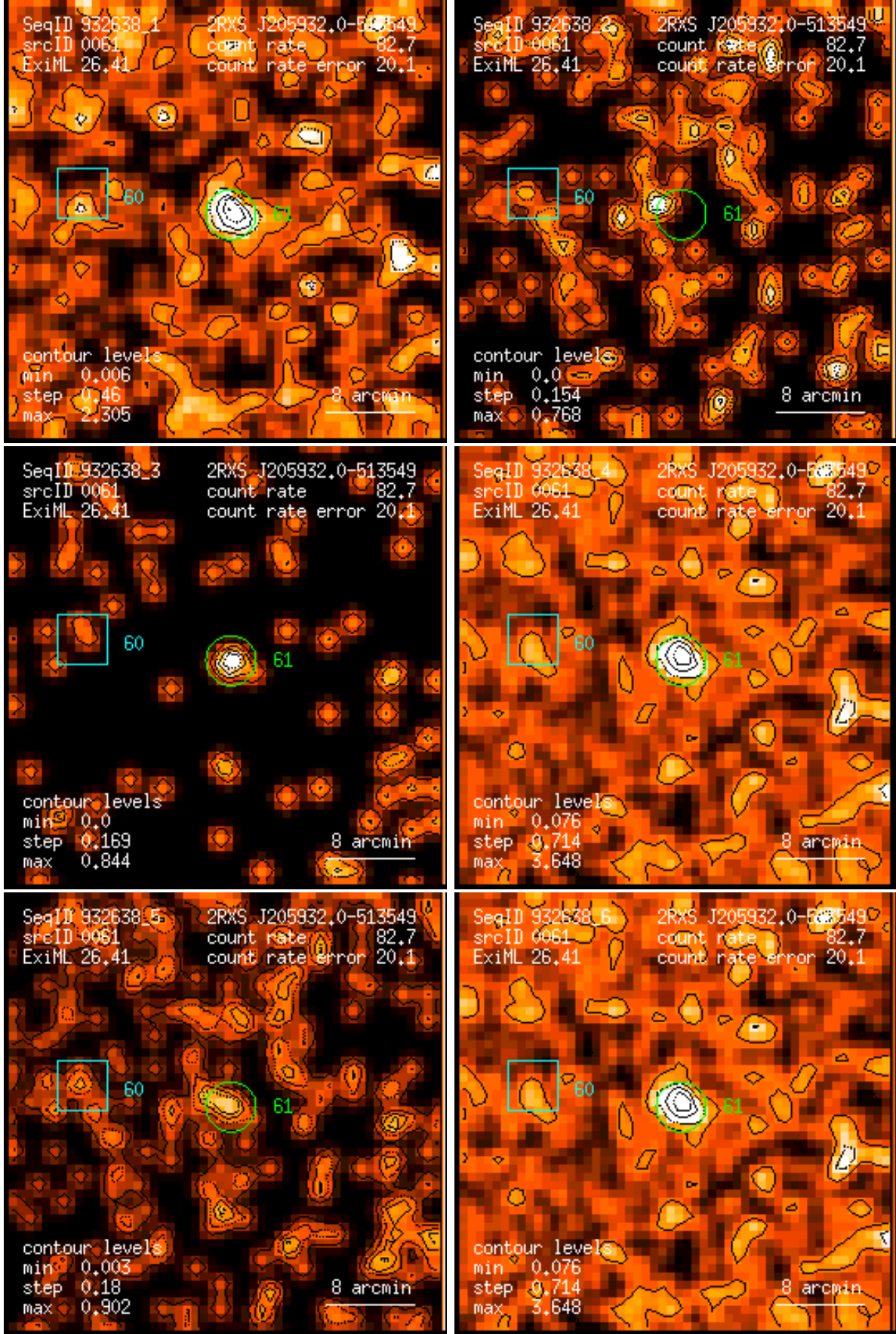
Figure 61: RASS 932638: detection 0061: band rate images, Gaussian filter: (1) PSPC channels 11 – 41, (2) 52 – 90, (3) 91 – 201, (4) 11 – 235, (5) 52 – 201, (6) 11 – 201. Broad band rates in counts/ks. Band rate contour levels in counts/ks/arcmin 2 .
