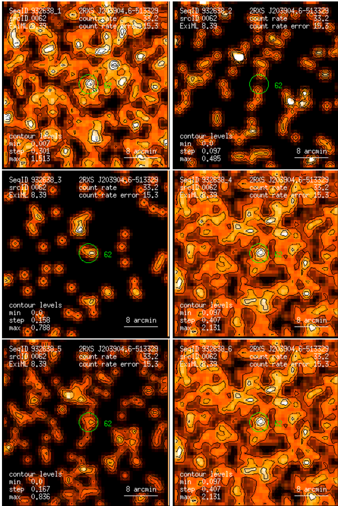
Figure 62: RASS 932638: detection 0062: band rate images, Gaussian filter: (1) PSPC channels 11 – 41, (2) 52 – 90, (3) 91 – 201, (4) 11 – 235, (5) 52 – 201, (6) 11 – 201. Broad band rates in counts/ks. Band rate contour levels in counts/ks/arcmin 2 .
