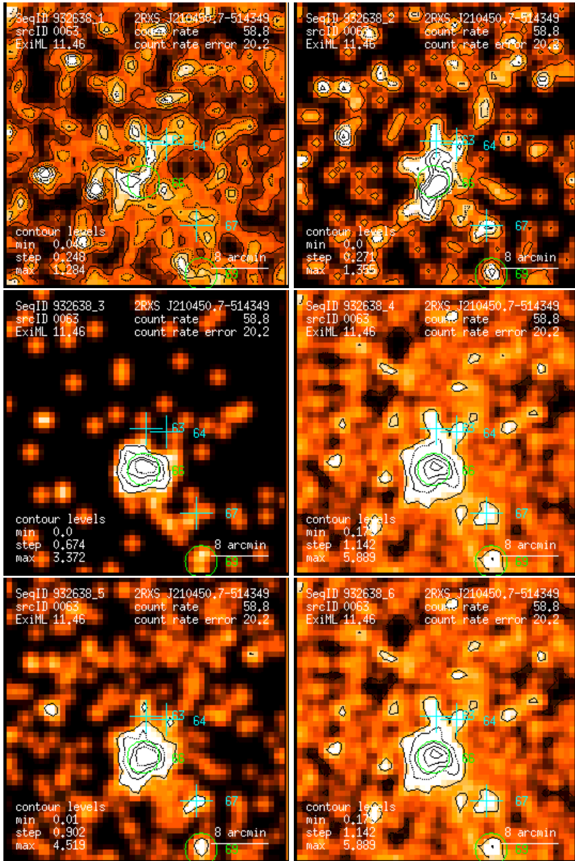
Figure 63: RASS 932638: detection 0063: band rate images, Gaussian filter: (1) PSPC channels 11 – 41, (2) 52 – 90, (3) 91 – 201, (4) 11 – 235, (5) 52 – 201, (6) 11 – 201. Broad band rates in counts/ks. Band rate contour levels in counts/ks/arcmin 2 .
