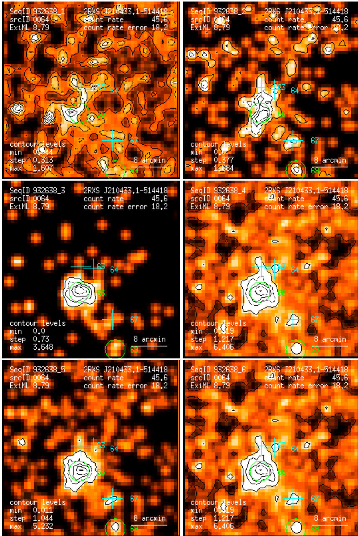
Figure 64: RASS 932638: detection 0064: band rate images, Gaussian filter: (1) PSPC channels 11 – 41, (2) 52 – 90, (3) 91 – 201, (4) 11 – 235, (5) 52 – 201, (6) 11 – 201. Broad band rates in counts/ks. Band rate contour levels in counts/ks/arcmin 2 .
