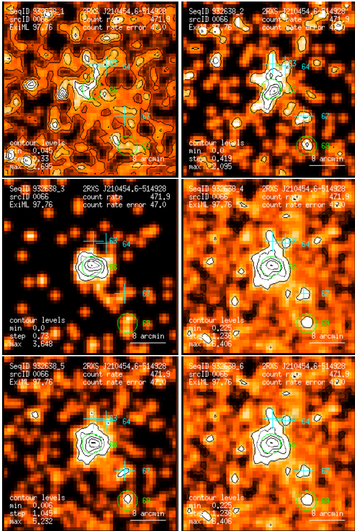
Figure 66: RASS 932638: detection 0066: band rate images, Gaussian filter: (1) PSPC channels 11 – 41, (2) 52 – 90, (3) 91 – 201, (4) 11 – 235, (5) 52 – 201, (6) 11 – 201. Broad band rates in counts/ks. Band rate contour levels in counts/ks/arcmin 2 .
