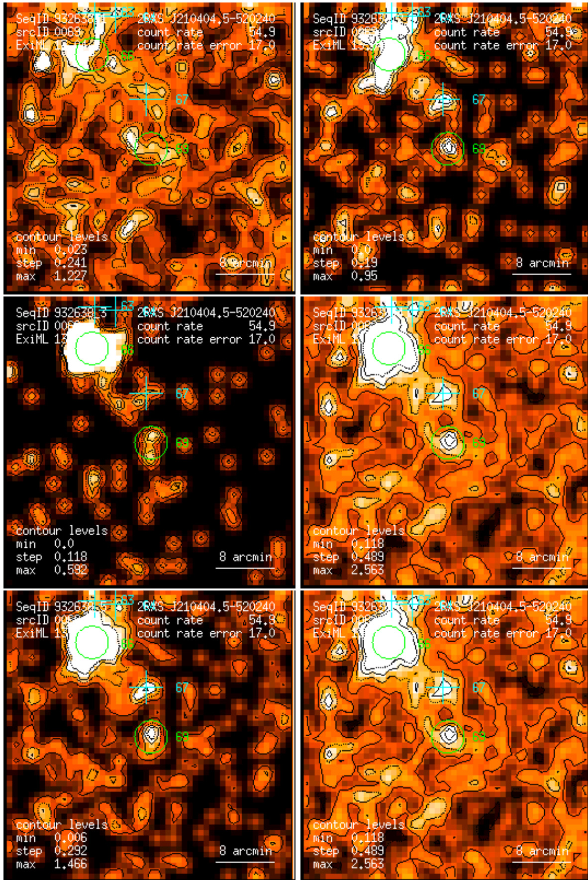
Figure 69: RASS 932638: detection 0069: band rate images, Gaussian filter: (1) PSPC channels 11 – 41, (2) 52 – 90, (3) 91 – 201, (4) 11 – 235, (5) 52 – 201, (6) 11 – 201. Broad band rates in counts/ks. Band rate contour levels in counts/ks/arcmin 2 .
