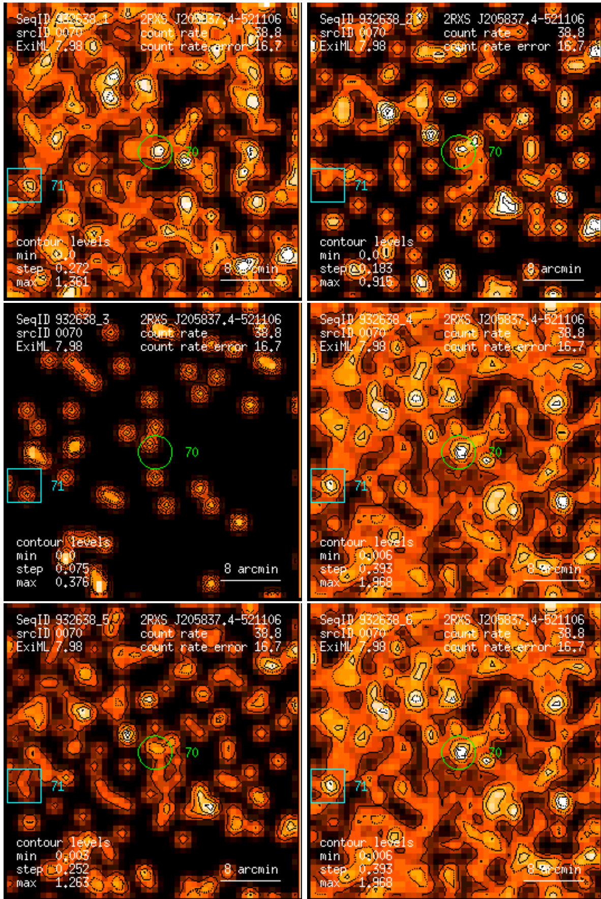
Figure 70: RASS 932638: detection 0070: band rate images, Gaussian filter: (1) PSPC channels 11 – 41, (2) 52 – 90, (3) 91 – 201, (4) 11 – 235, (5) 52 – 201, (6) 11 – 201. Broad band rates in counts/ks. Band rate contour levels in counts/ks/arcmin 2 .
