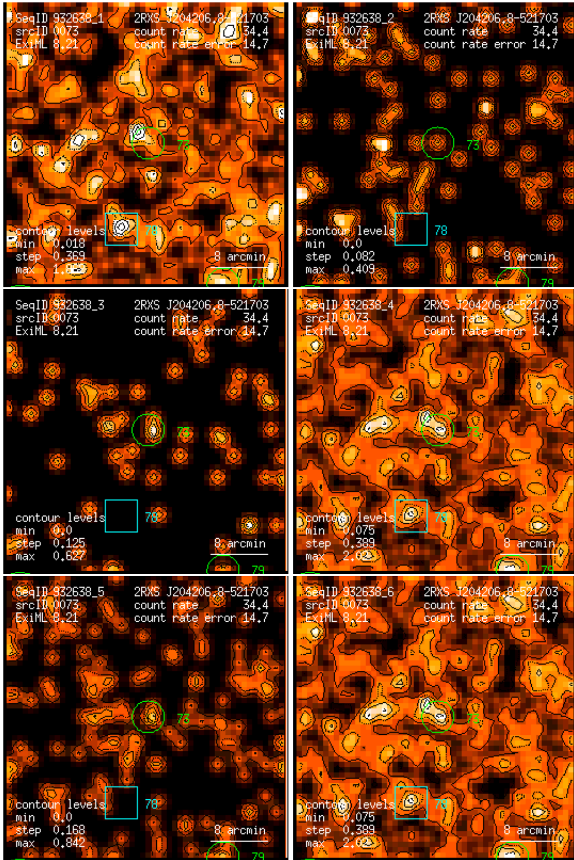
Figure 73: RASS 932638: detection 0073: band rate images, Gaussian filter: (1) PSPC channels 11 – 41, (2) 52 – 90, (3) 91 – 201, (4) 11 – 235, (5) 52 – 201, (6) 11 – 201. Broad band rates in counts/ks. Band rate contour levels in counts/ks/arcmin 2 .
