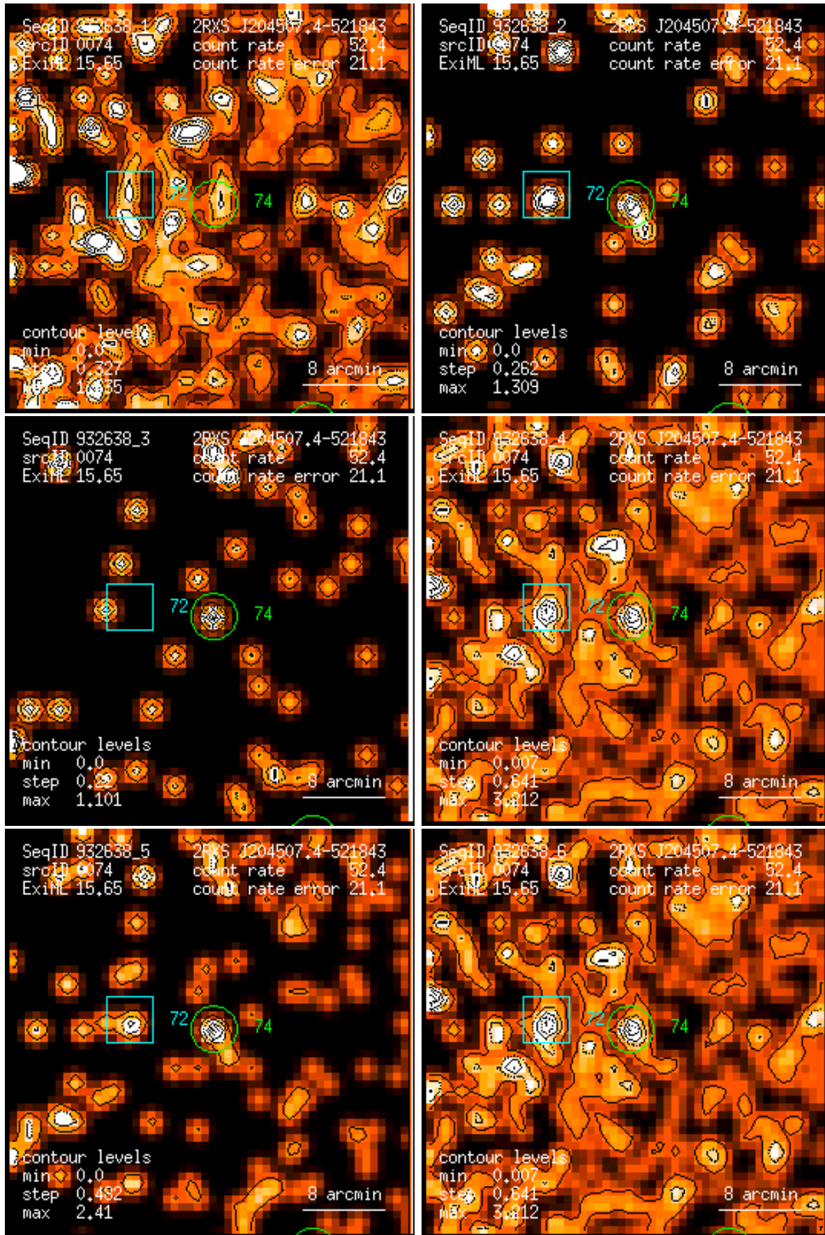
Figure 74: RASS 932638: detection 0074: band rate images, Gaussian filter: (1) PSPC channels 11 – 41, (2) 52 – 90, (3) 91 – 201, (4) 11 – 235, (5) 52 – 201, (6) 11 – 201. Broad band rates in counts/ks. Band rate contour levels in counts/ks/arcmin 2 .
