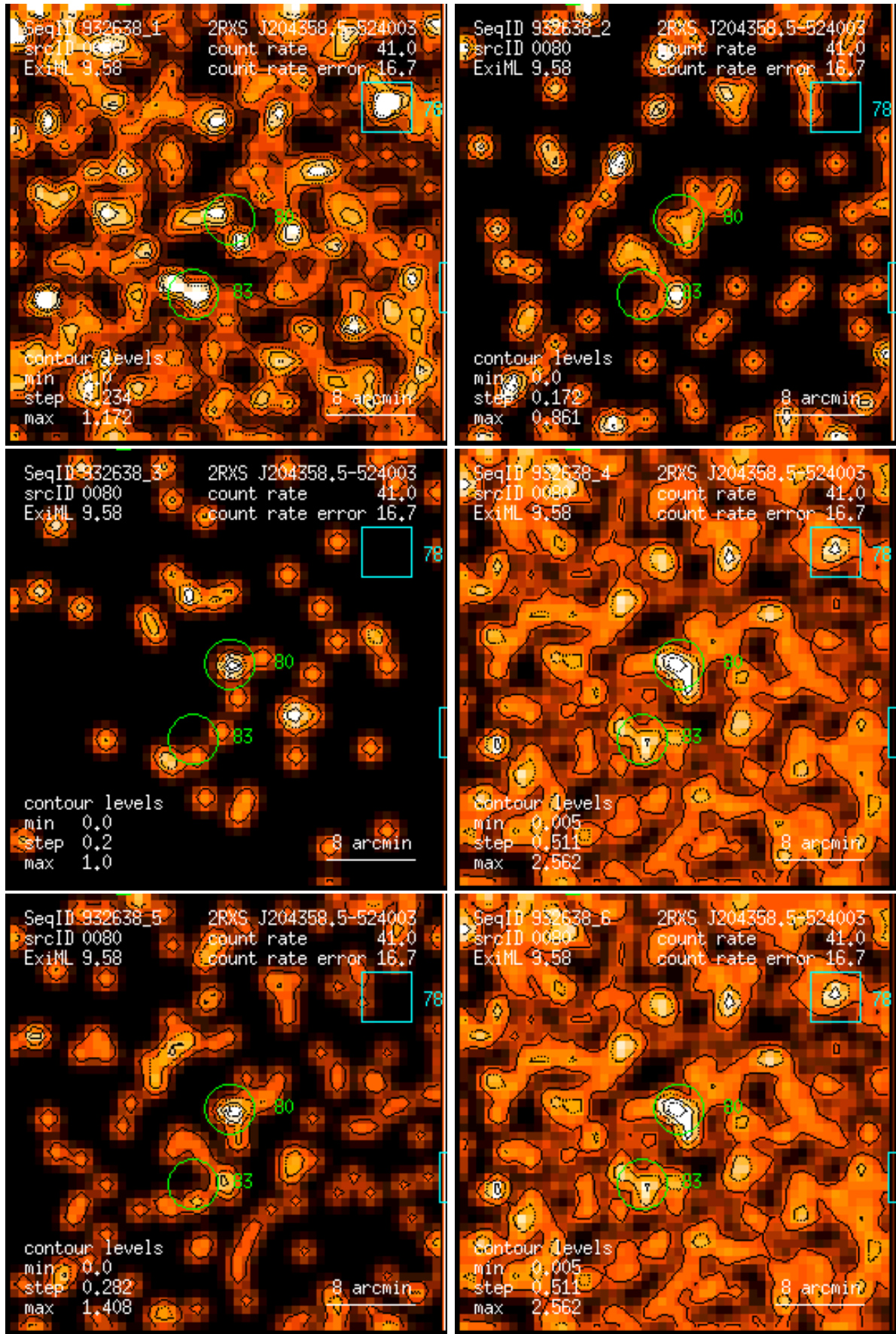
Figure 80: RASS 932638: detection 0080: band rate images, Gaussian filter: (1) PSPC channels 11 – 41, (2) 52 – 90, (3) 91 – 201, (4) 11 – 235, (5) 52 – 201, (6) 11 – 201. Broad band rates in counts/ks. Band rate contour levels in counts/ks/arcmin 2 .
