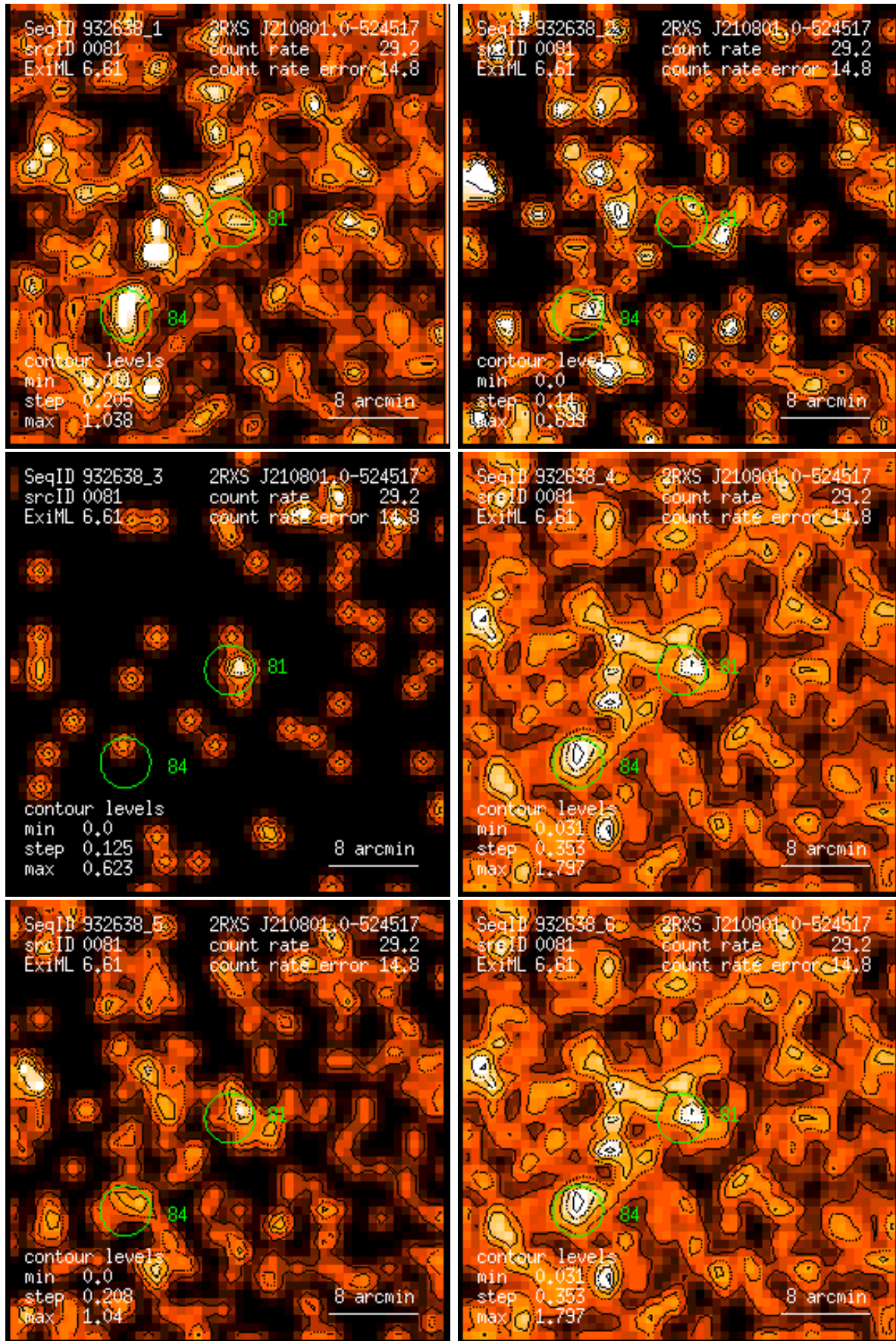
Figure 81: RASS 932638: detection 0081: band rate images, Gaussian filter: (1) PSPC channels 11 – 41, (2) 52 – 90, (3) 91 – 201, (4) 11 – 235, (5) 52 – 201, (6) 11 – 201. Broad band rates in counts/ks. Band rate contour levels in counts/ks/arcmin 2 .
