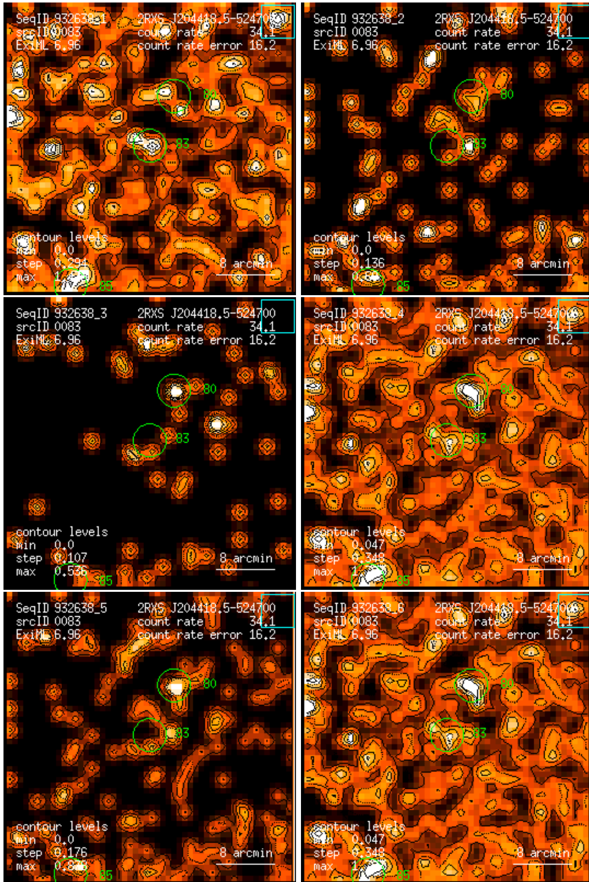
Figure 83: RASS 932638: detection 0083: band rate images, Gaussian filter: (1) PSPC channels 11 – 41, (2) 52 – 90, (3) 91 – 201, (4) 11 – 235, (5) 52 – 201, (6) 11 – 201. Broad band rates in counts/ks. Band rate contour levels in counts/ks/arcmin 2 .
