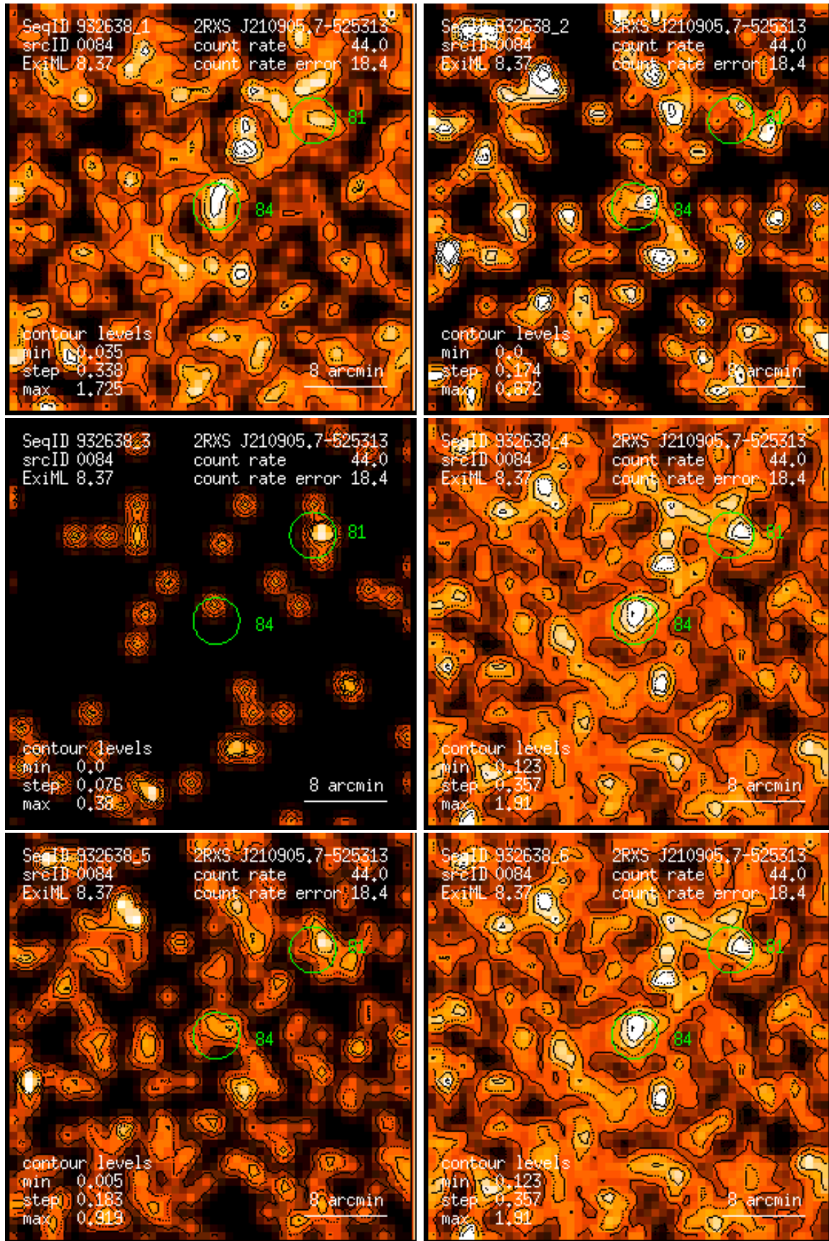
Figure 84: RASS 932638: detection 0084: band rate images, Gaussian filter: (1) PSPC channels 11 – 41, (2) 52 – 90, (3) 91 – 201, (4) 11 – 235, (5) 52 – 201, (6) 11 – 201. Broad band rates in counts/ks. Band rate contour levels in counts/ks/arcmin 2 .
