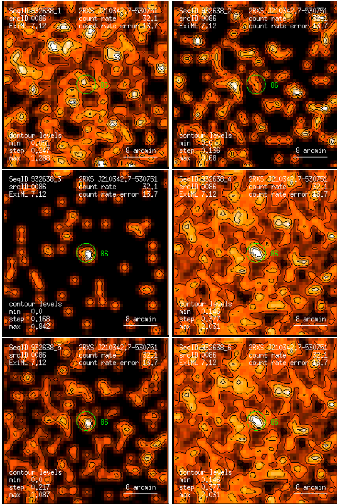
Figure 86: RASS 932638: detection 0086: band rate images, Gaussian filter: (1) PSPC channels 11 – 41, (2) 52 – 90, (3) 91 – 201, (4) 11 – 235, (5) 52 – 201, (6) 11 – 201. Broad band rates in counts/ks. Band rate contour levels in counts/ks/arcmin 2 .
