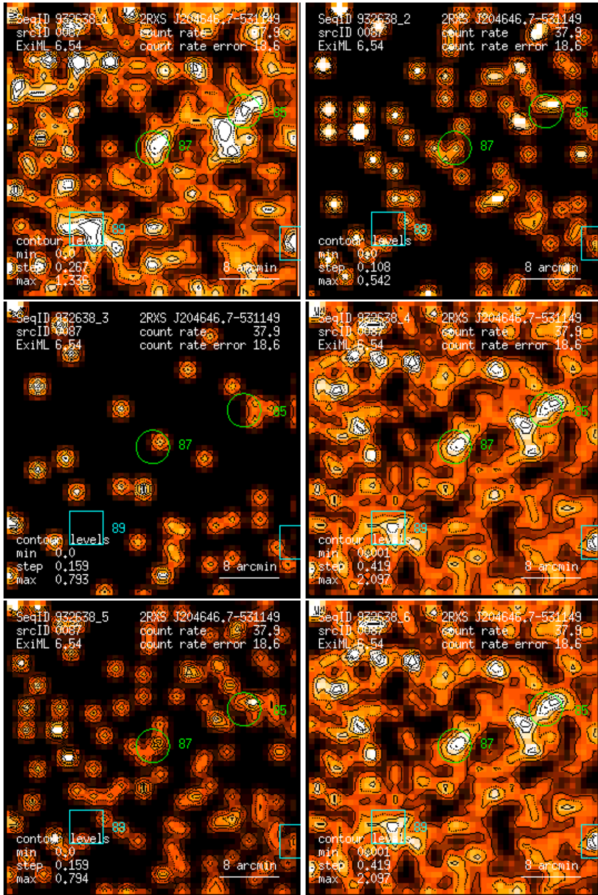
Figure 87: RASS 932638: detection 0087: band rate images, Gaussian filter: (1) PSPC channels 11 – 41, (2) 52 – 90, (3) 91 – 201, (4) 11 – 235, (5) 52 – 201, (6) 11 – 201. Broad band rates in counts/ks. Band rate contour levels in counts/ks/arcmin 2 .
