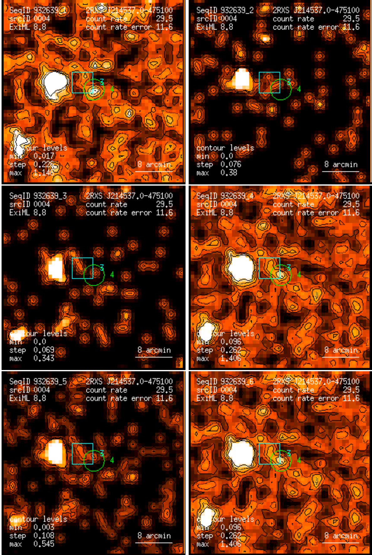
Figure 4: RASS 932639: detection 0004: band rate images, Gaussian filter: (1) PSPC channels 11 – 41, (2) 52 – 90, (3) 91 – 201, (4) 11 – 235, (5) 52 – 201, (6) 11 – 201. Broad band rates in counts/ks. Band rate contour levels in counts/ks/arcmin 2 .
