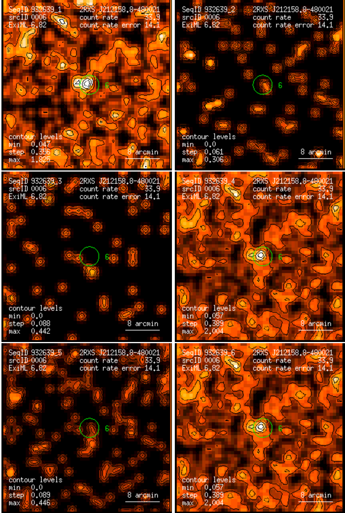
Figure 6: RASS 932639: detection 0006: band rate images, Gaussian filter: (1) PSPC channels 11 – 41, (2) 52 – 90, (3) 91 – 201, (4) 11 – 235, (5) 52 – 201, (6) 11 – 201. Broad band rates in counts/ks. Band rate contour levels in counts/ks/arcmin 2 .
