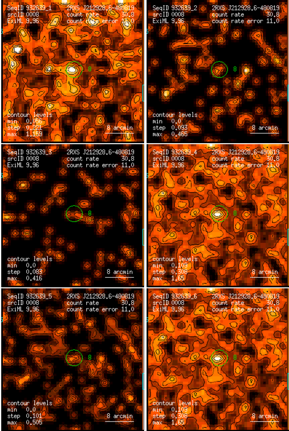
Figure 8: RASS 932639: detection 0008: band rate images, Gaussian filter: (1) PSPC channels 11 – 41, (2) 52 – 90, (3) 91 – 201, (4) 11 – 235, (5) 52 – 201, (6) 11 – 201. Broad band rates in counts/ks. Band rate contour levels in counts/ks/arcmin 2 .
