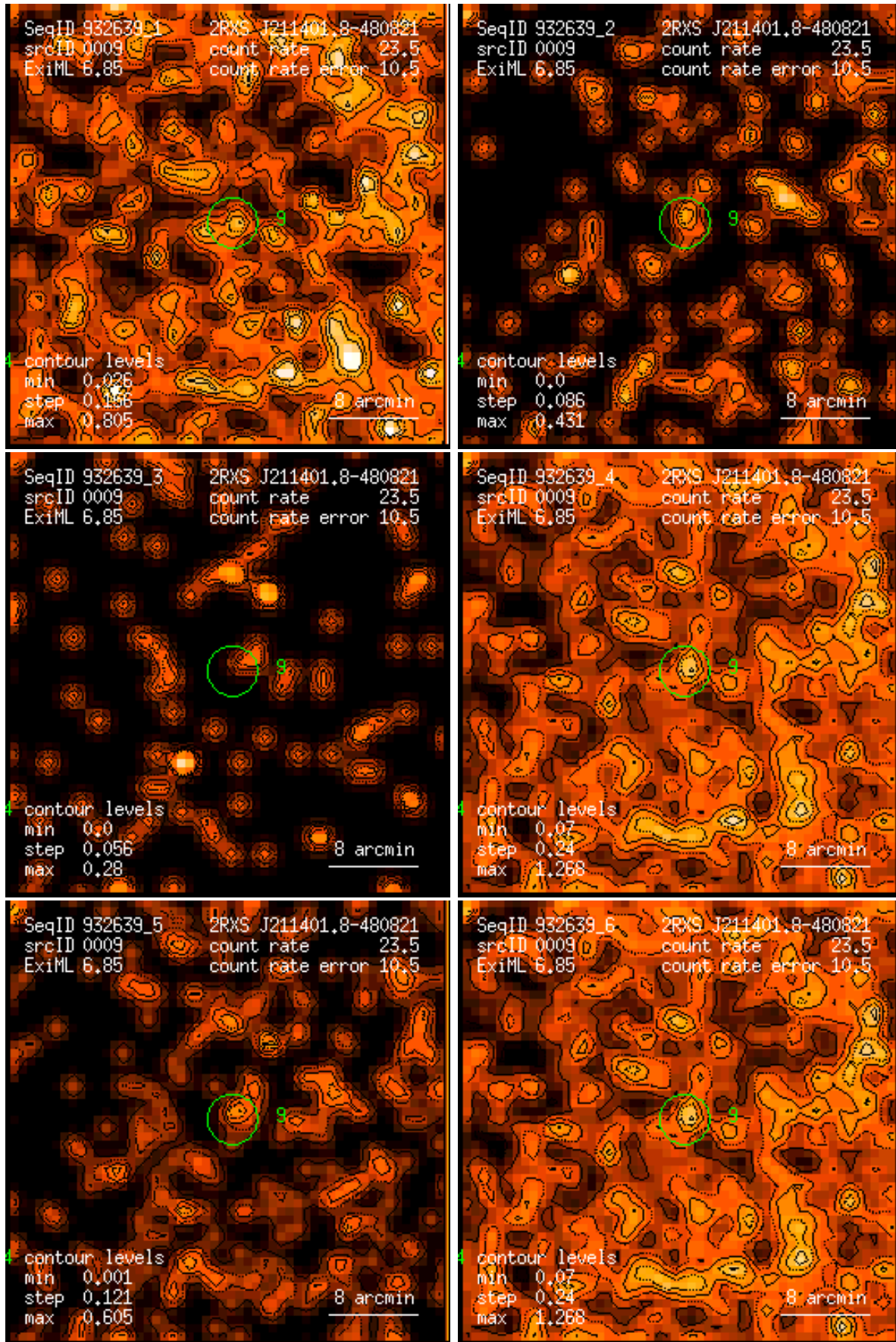
Figure 9: RASS 932639: detection 0009: band rate images, Gaussian filter: (1) PSPC channels 11 – 41, (2) 52 – 90, (3) 91 – 201, (4) 11 – 235, (5) 52 – 201, (6) 11 – 201. Broad band rates in counts/ks. Band rate contour levels in counts/ks/arcmin 2 .
