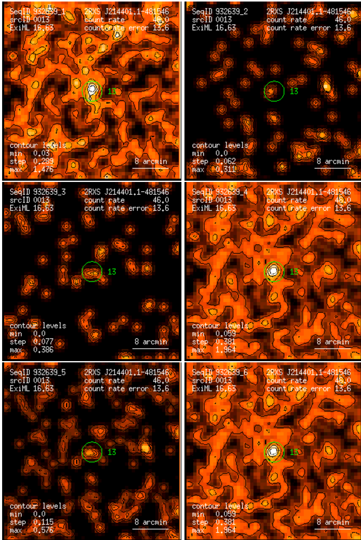
Figure 13: RASS 932639: detection 0013: band rate images, Gaussian filter: (1) PSPC channels 11 – 41, (2) 52 – 90, (3) 91 – 201, (4) 11 – 235, (5) 52 – 201, (6) 11 – 201. Broad band rates in counts/ks. Band rate contour levels in counts/ks/arcmin 2 .
