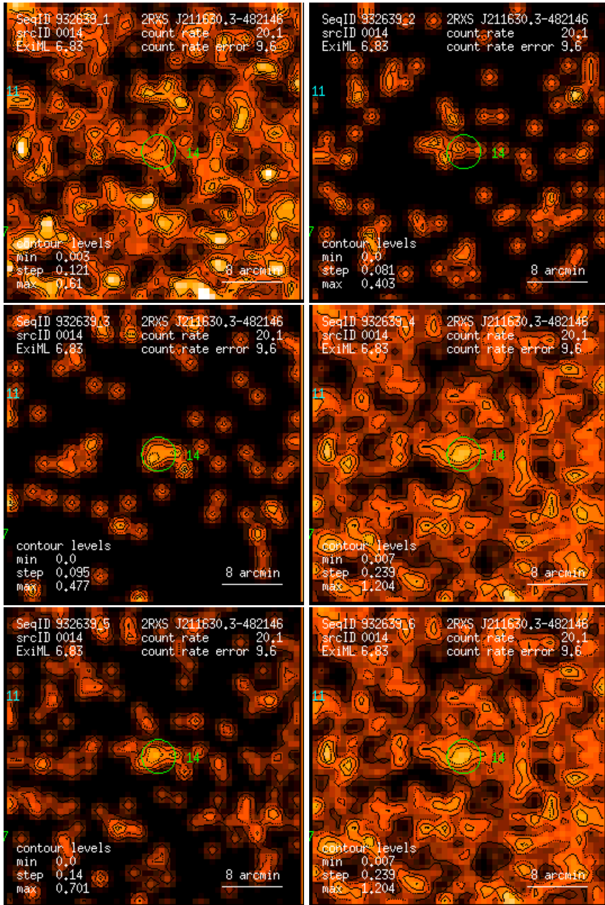
Figure 14: RASS 932639: detection 0014: band rate images, Gaussian filter: (1) PSPC channels 11 – 41, (2) 52 – 90, (3) 91 – 201, (4) 11 – 235, (5) 52 – 201, (6) 11 – 201. Broad band rates in counts/ks. Band rate contour levels in counts/ks/arcmin 2 .
