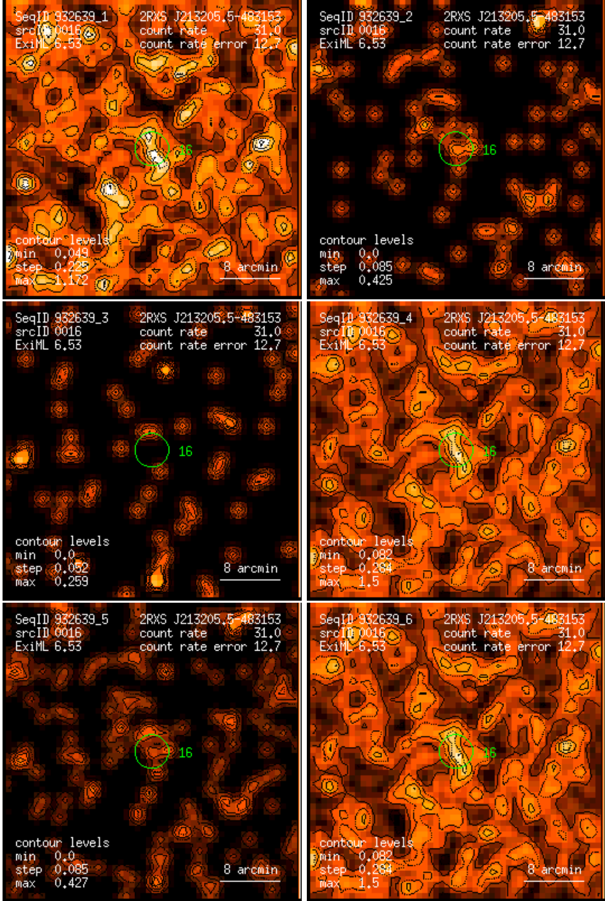
Figure 16: RASS 932639: detection 0016: band rate images, Gaussian filter: (1) PSPC channels 11 – 41, (2) 52 – 90, (3) 91 – 201, (4) 11 – 235, (5) 52 – 201, (6) 11 – 201. Broad band rates in counts/ks. Band rate contour levels in counts/ks/arcmin 2 .
