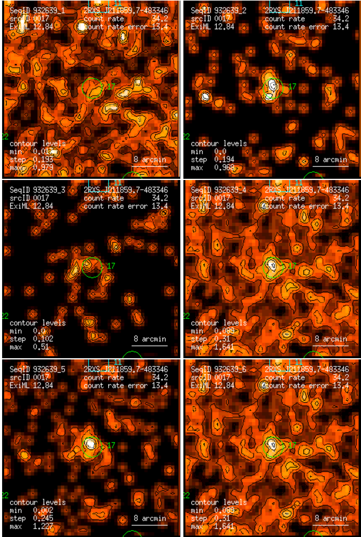
Figure 17: RASS 932639: detection 0017: band rate images, Gaussian filter: (1) PSPC channels 11 – 41, (2) 52 – 90, (3) 91 – 201, (4) 11 – 235, (5) 52 – 201, (6) 11 – 201. Broad band rates in counts/ks. Band rate contour levels in counts/ks/arcmin 2 .
