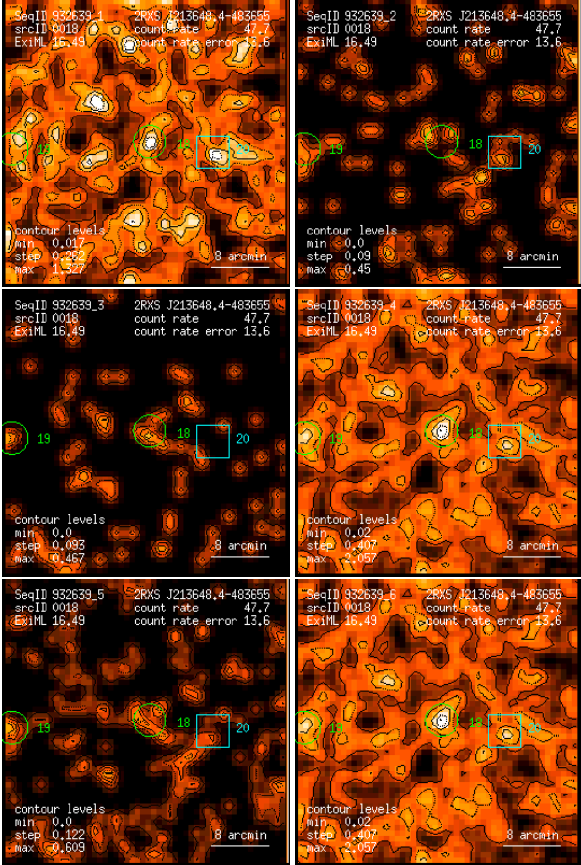
Figure 18: RASS 932639: detection 0018: band rate images, Gaussian filter: (1) PSPC channels 11 – 41, (2) 52 – 90, (3) 91 – 201, (4) 11 – 235, (5) 52 – 201, (6) 11 – 201. Broad band rates in counts/ks. Band rate contour levels in counts/ks/arcmin 2 .
