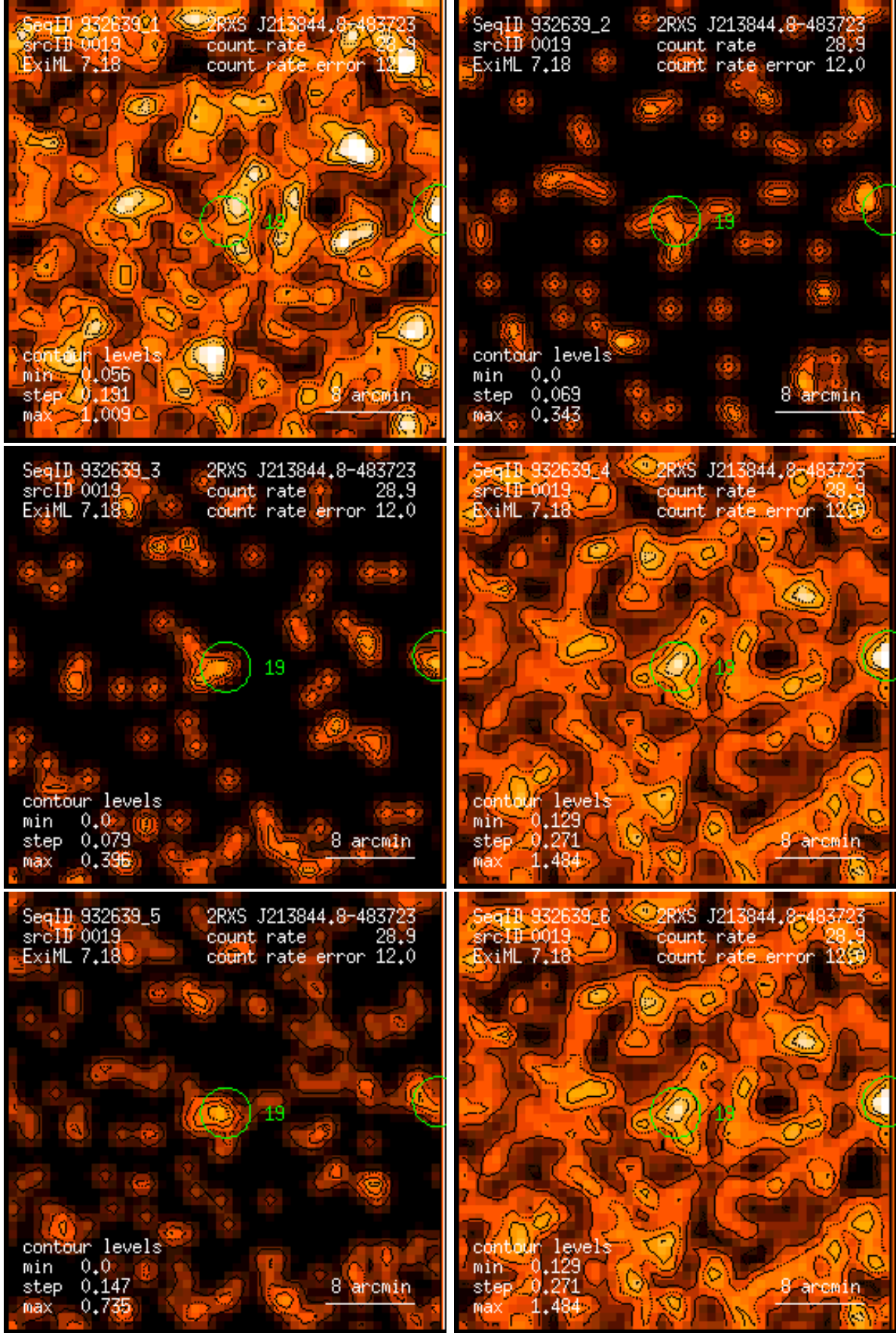
Figure 19: RASS 932639: detection 0019: band rate images, Gaussian filter: (1) PSPC channels 11 – 41, (2) 52 – 90, (3) 91 – 201, (4) 11 – 235, (5) 52 – 201, (6) 11 – 201. Broad band rates in counts/ks. Band rate contour levels in counts/ks/arcmin 2 .
