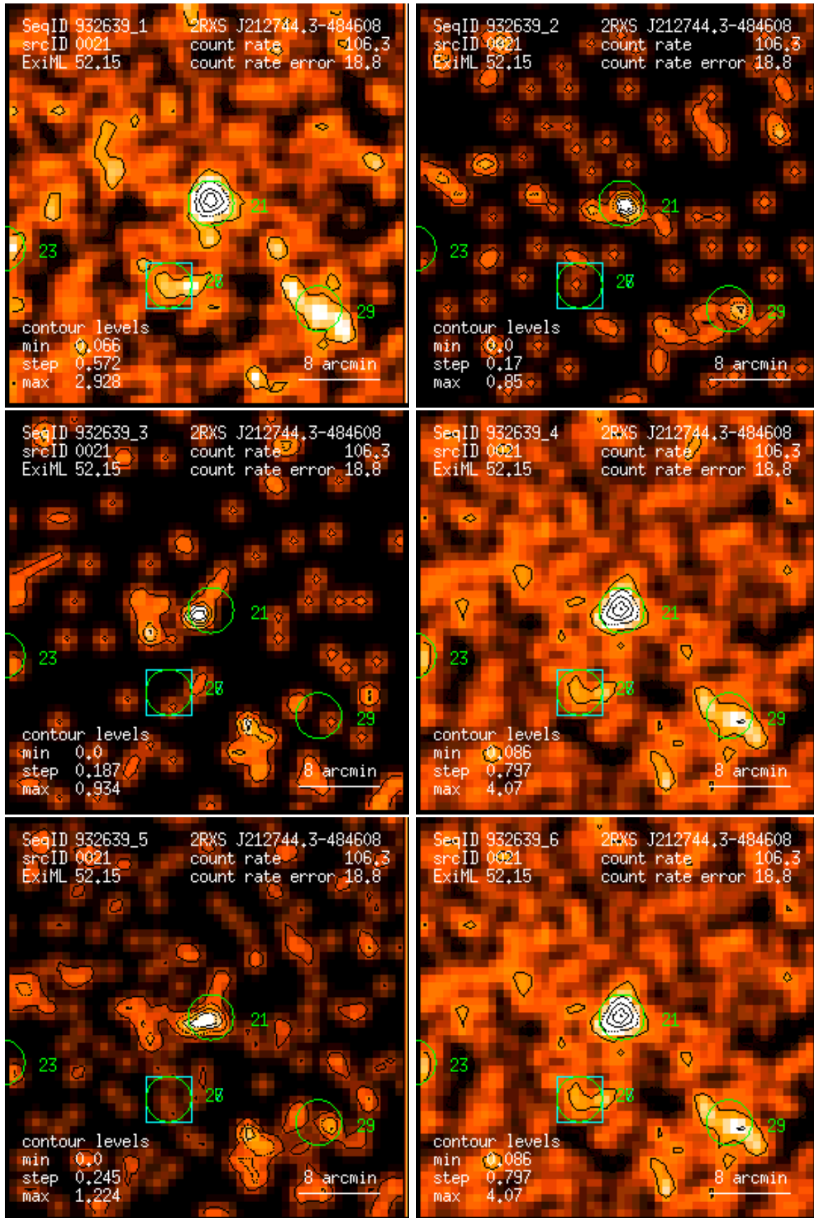
Figure 21: RASS 932639: detection 0021: band rate images, Gaussian filter: (1) PSPC channels 11 – 41, (2) 52 – 90, (3) 91 – 201, (4) 11 – 235, (5) 52 – 201, (6) 11 – 201. Broad band rates in counts/ks. Band rate contour levels in counts/ks/arcmin 2 .
