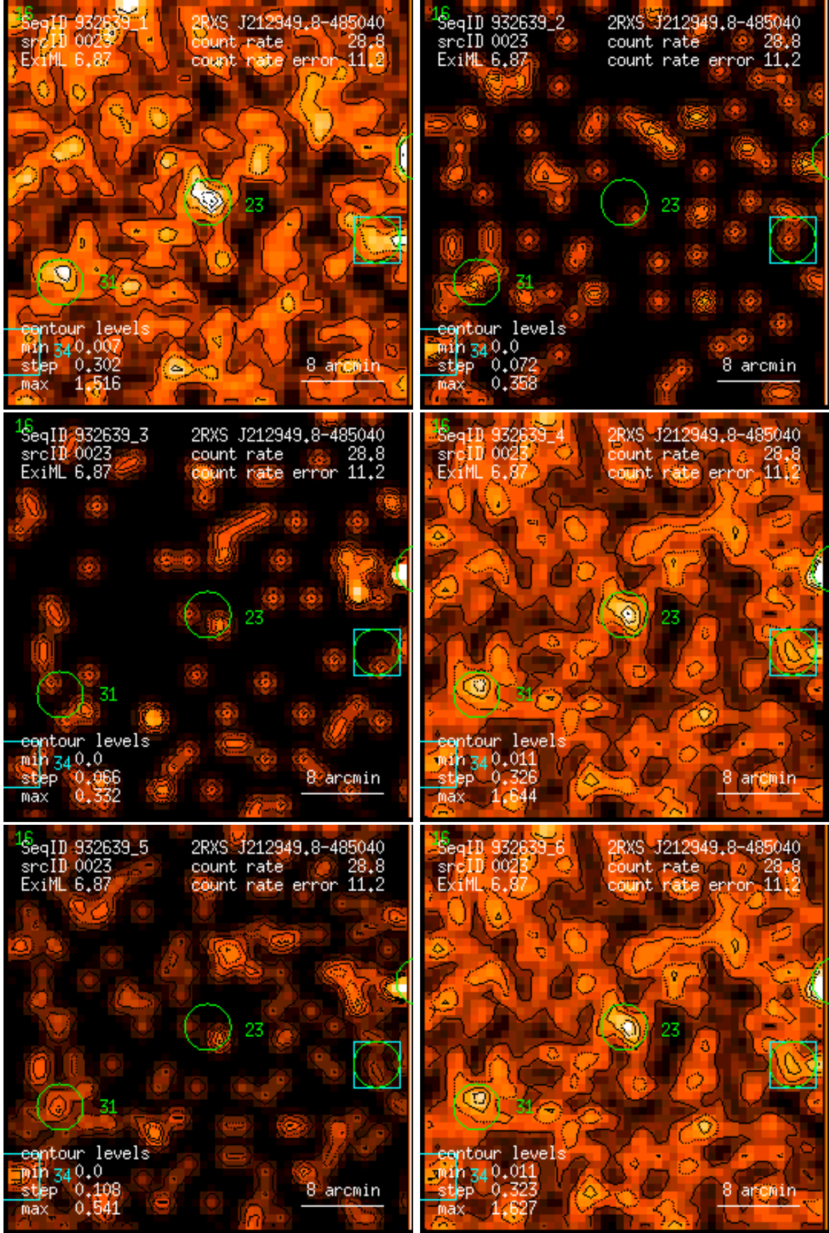
Figure 23: RASS 932639: detection 0023: band rate images, Gaussian filter: (1) PSPC channels 11 – 41, (2) 52 – 90, (3) 91 – 201, (4) 11 – 235, (5) 52 – 201, (6) 11 – 201. Broad band rates in counts/ks. Band rate contour levels in counts/ks/arcmin 2 .
