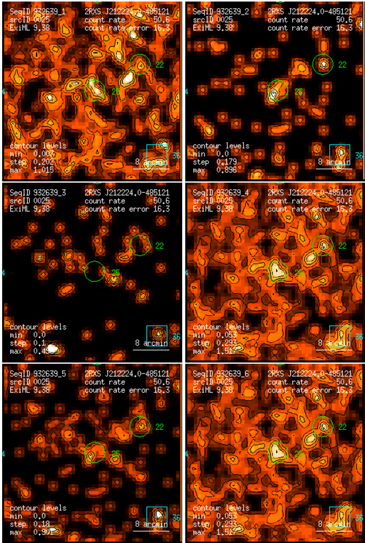
Figure 25: RASS 932639: detection 0025: band rate images, Gaussian filter: (1) PSPC channels 11 – 41, (2) 52 – 90, (3) 91 – 201, (4) 11 – 235, (5) 52 – 201, (6) 11 – 201. Broad band rates in counts/ks. Band rate contour levels in counts/ks/arcmin 2 .
