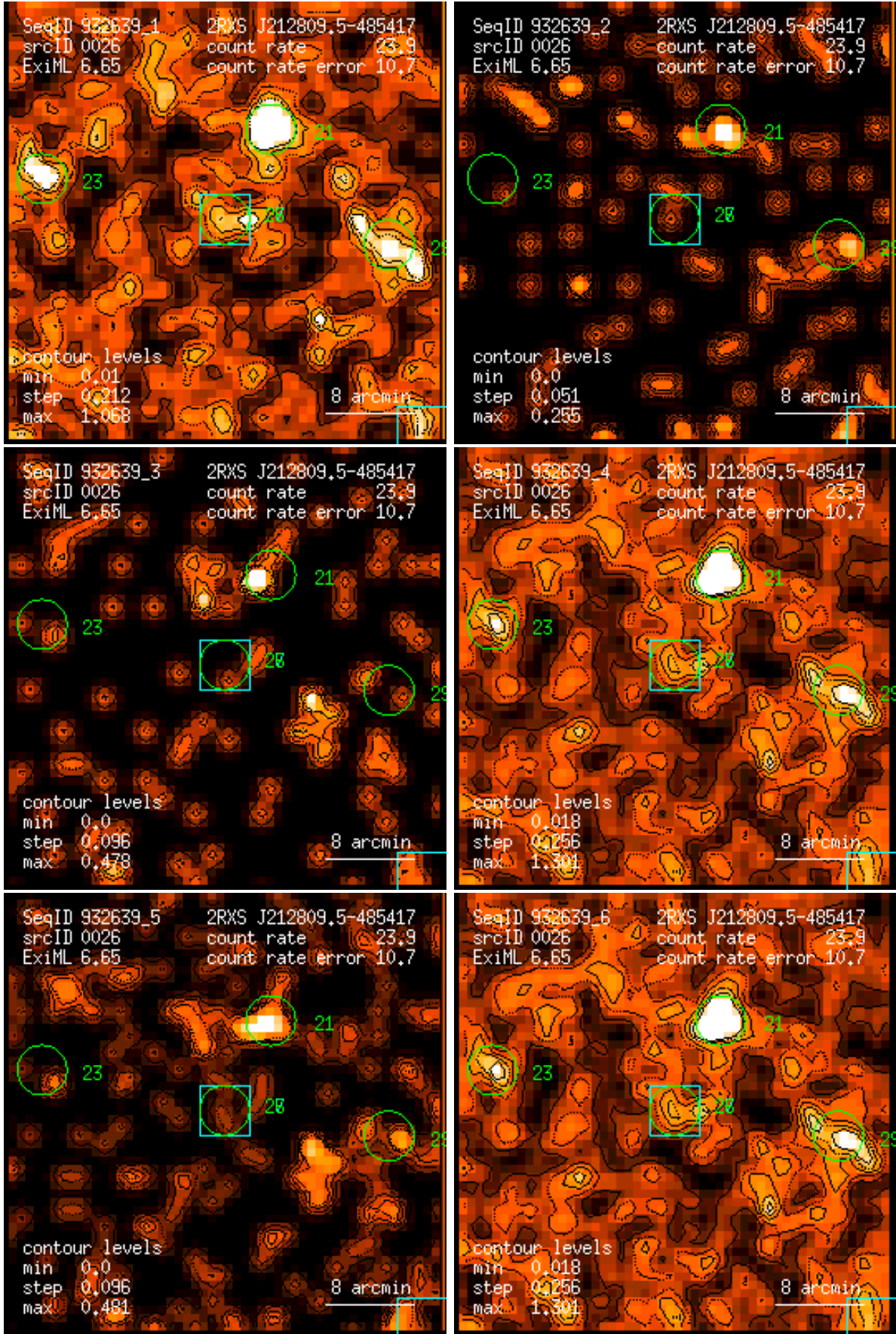
Figure 26: RASS 932639: detection 0026: band rate images, Gaussian filter: (1) PSPC channels 11 – 41, (2) 52 – 90, (3) 91 – 201, (4) 11 – 235, (5) 52 – 201, (6) 11 – 201. Broad band rates in counts/ks. Band rate contour levels in counts/ks/arcmin 2 .
