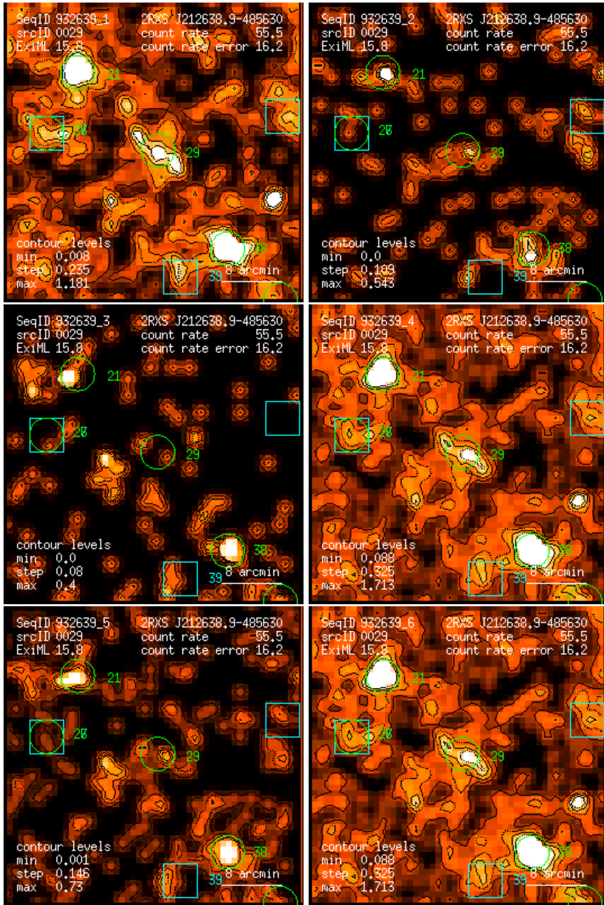
Figure 29: RASS 932639: detection 0029: band rate images, Gaussian filter: (1) PSPC channels 11 – 41, (2) 52 – 90, (3) 91 – 201, (4) 11 – 235, (5) 52 – 201, (6) 11 – 201. Broad band rates in counts/ks. Band rate contour levels in counts/ks/arcmin 2 .
