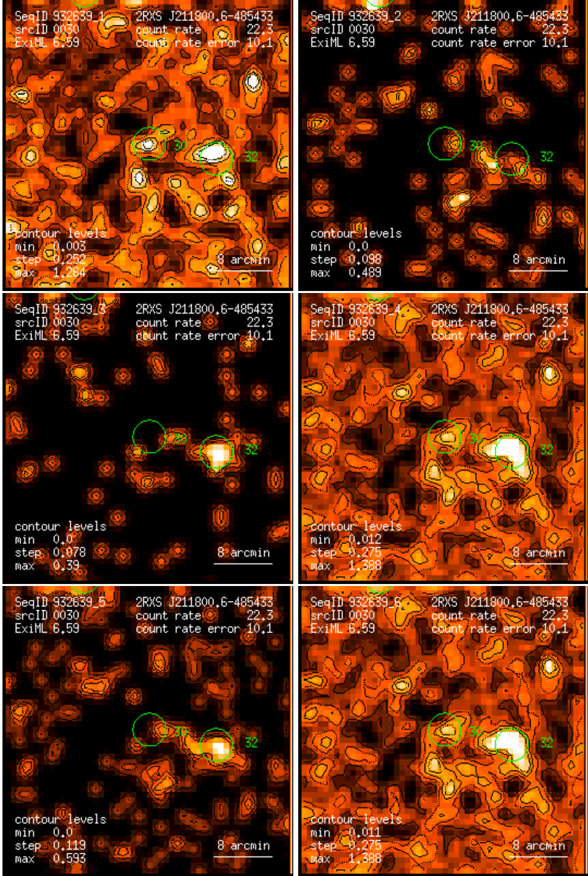
Figure 30: RASS 932639: detection 0030: band rate images, Gaussian filter: (1) PSPC channels 11 – 41, (2) 52 – 90, (3) 91 – 201, (4) 11 – 235, (5) 52 – 201, (6) 11 – 201. Broad band rates in counts/ks. Band rate contour levels in counts/ks/arcmin 2 .
