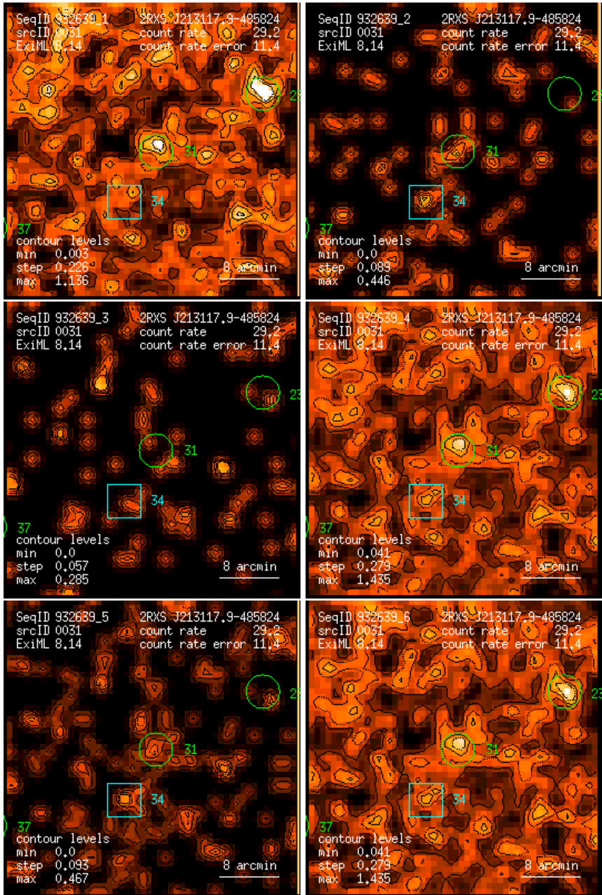
Figure 31: RASS 932639: detection 0031: band rate images, Gaussian filter: (1) PSPC channels 11 – 41, (2) 52 – 90, (3) 91 – 201, (4) 11 – 235, (5) 52 – 201, (6) 11 – 201. Broad band rates in counts/ks. Band rate contour levels in counts/ks/arcmin 2 .
