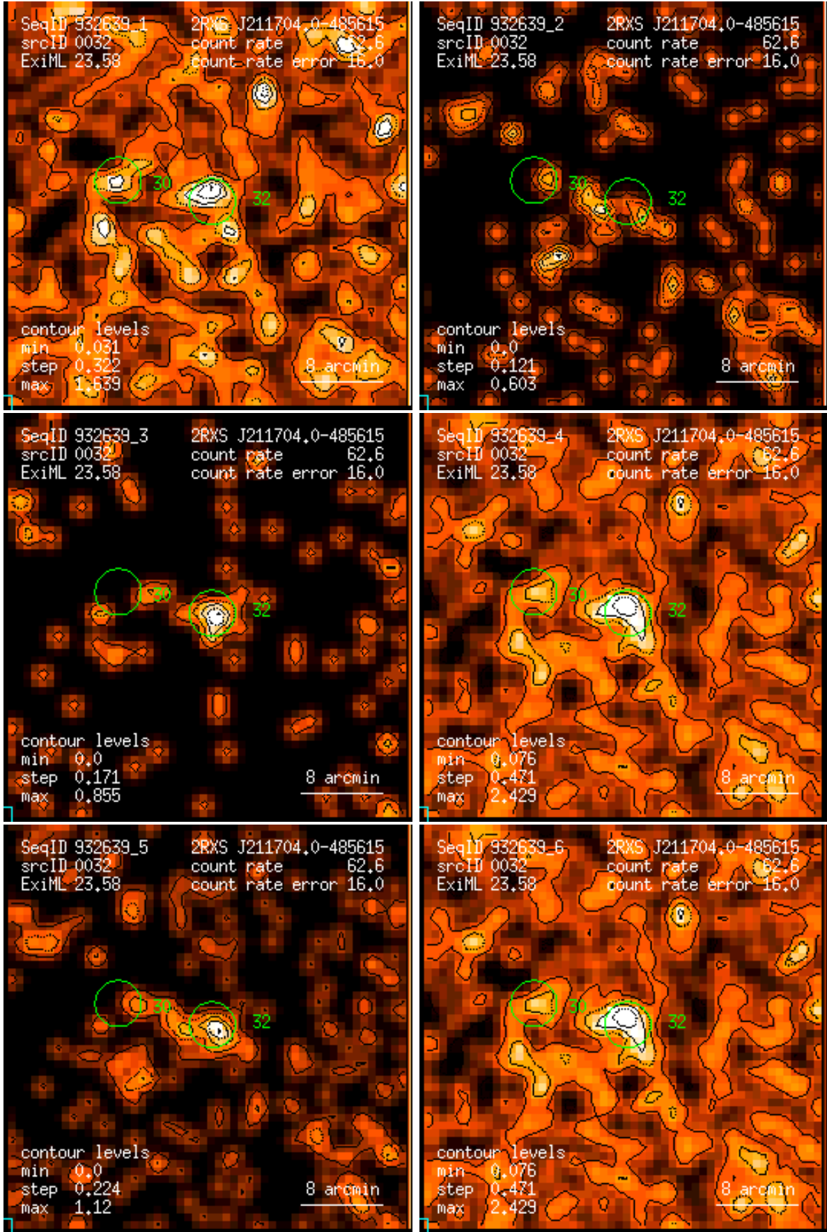
Figure 32: RASS 932639: detection 0032: band rate images, Gaussian filter: (1) PSPC channels 11 – 41, (2) 52 – 90, (3) 91 – 201, (4) 11 – 235, (5) 52 – 201, (6) 11 – 201. Broad band rates in counts/ks. Band rate contour levels in counts/ks/arcmin 2 .
