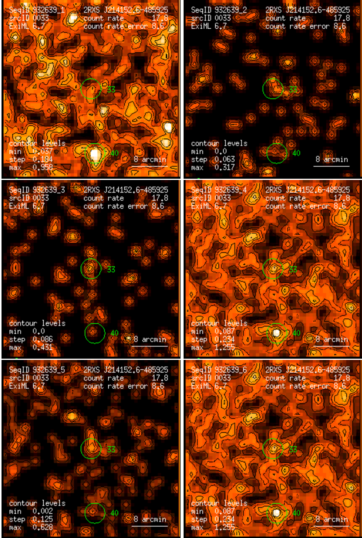
Figure 33: RASS 932639: detection 0033: band rate images, Gaussian filter: (1) PSPC channels 11 – 41, (2) 52 – 90, (3) 91 – 201, (4) 11 – 235, (5) 52 – 201, (6) 11 – 201. Broad band rates in counts/ks. Band rate contour levels in counts/ks/arcmin 2 .
