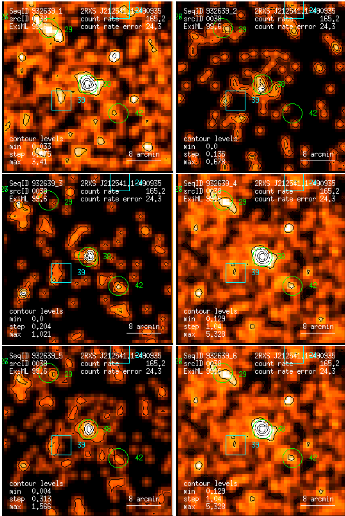
Figure 38: RASS 932639: detection 0038: band rate images, Gaussian filter: (1) PSPC channels 11 – 41, (2) 52 – 90, (3) 91 – 201, (4) 11 – 235, (5) 52 – 201, (6) 11 – 201. Broad band rates in counts/ks. Band rate contour levels in counts/ks/arcmin 2 .
