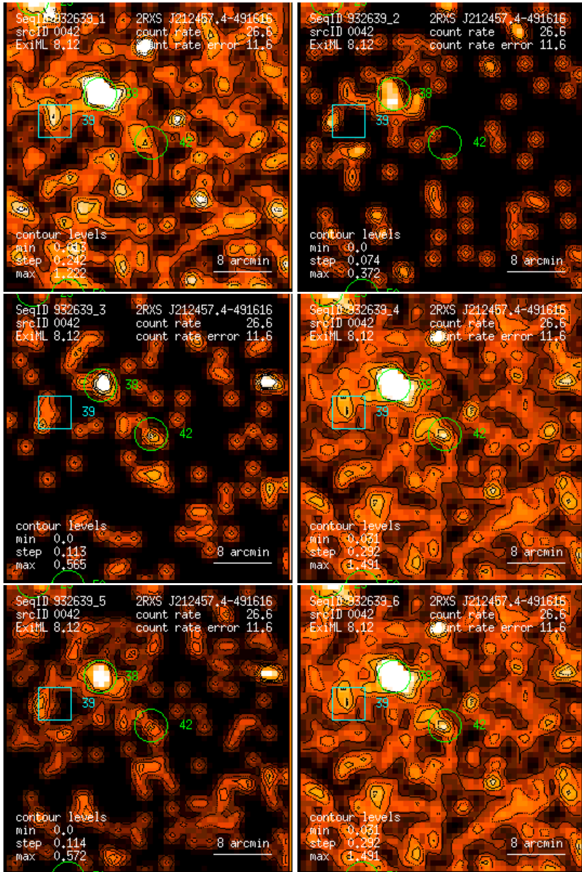
Figure 42: RASS 932639: detection 0042: band rate images, Gaussian filter: (1) PSPC channels 11 – 41, (2) 52 – 90, (3) 91 – 201, (4) 11 – 235, (5) 52 – 201, (6) 11 – 201. Broad band rates in counts/ks. Band rate contour levels in counts/ks/arcmin 2 .
