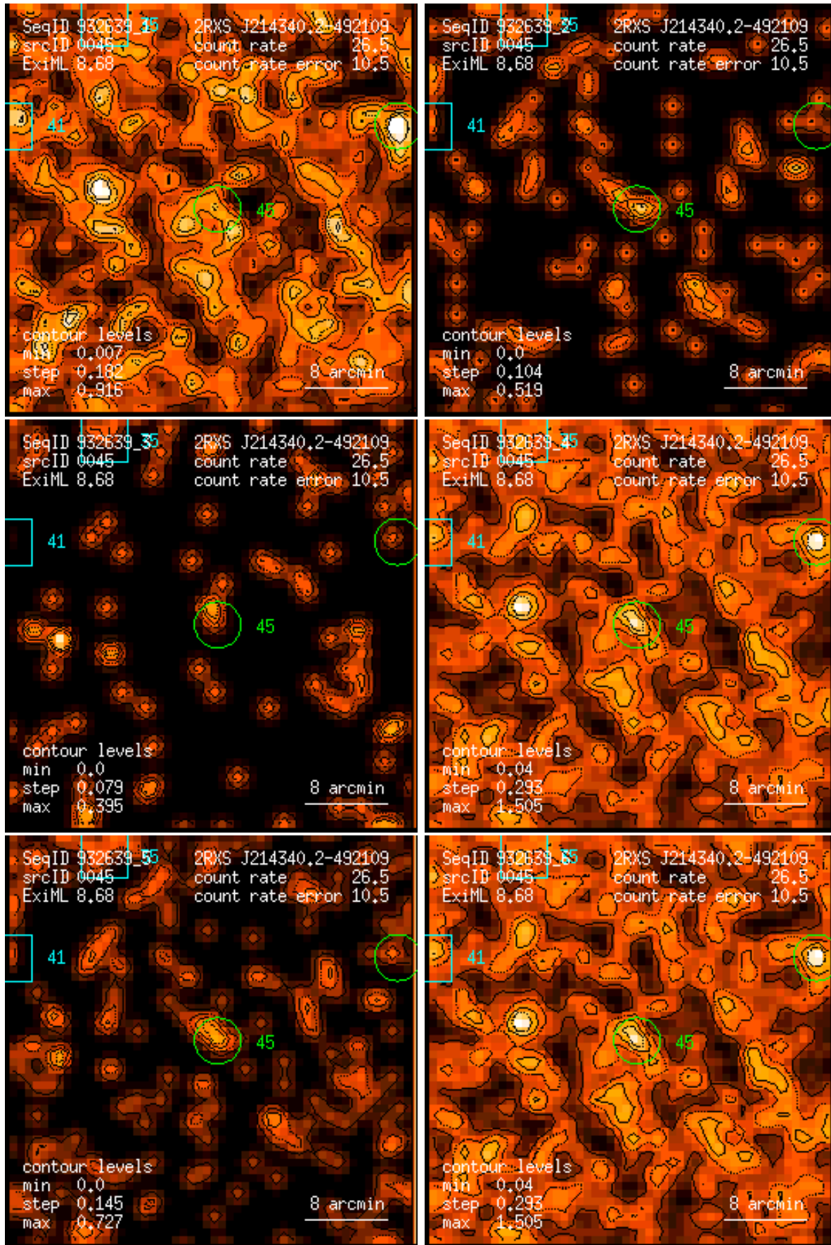
Figure 45: RASS 932639: detection 0045: band rate images, Gaussian filter: (1) PSPC channels 11 – 41, (2) 52 – 90, (3) 91 – 201, (4) 11 – 235, (5) 52 – 201, (6) 11 – 201. Broad band rates in counts/ks. Band rate contour levels in counts/ks/arcmin 2 .
