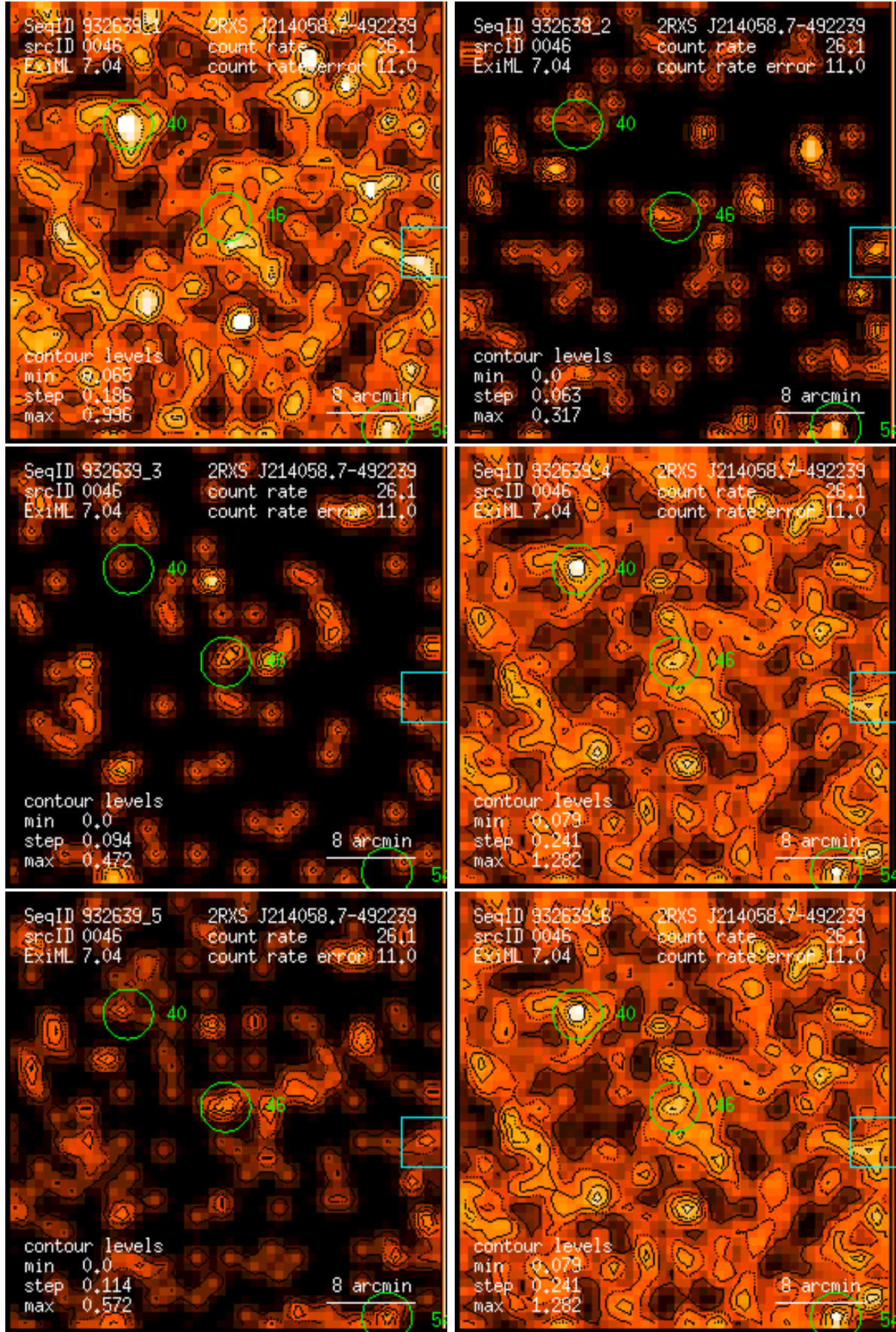
Figure 46: RASS 932639: detection 0046: band rate images, Gaussian filter: (1) PSPC channels 11 – 41, (2) 52 – 90, (3) 91 – 201, (4) 11 – 235, (5) 52 – 201, (6) 11 – 201. Broad band rates in counts/ks. Band rate contour levels in counts/ks/arcmin 2 .
