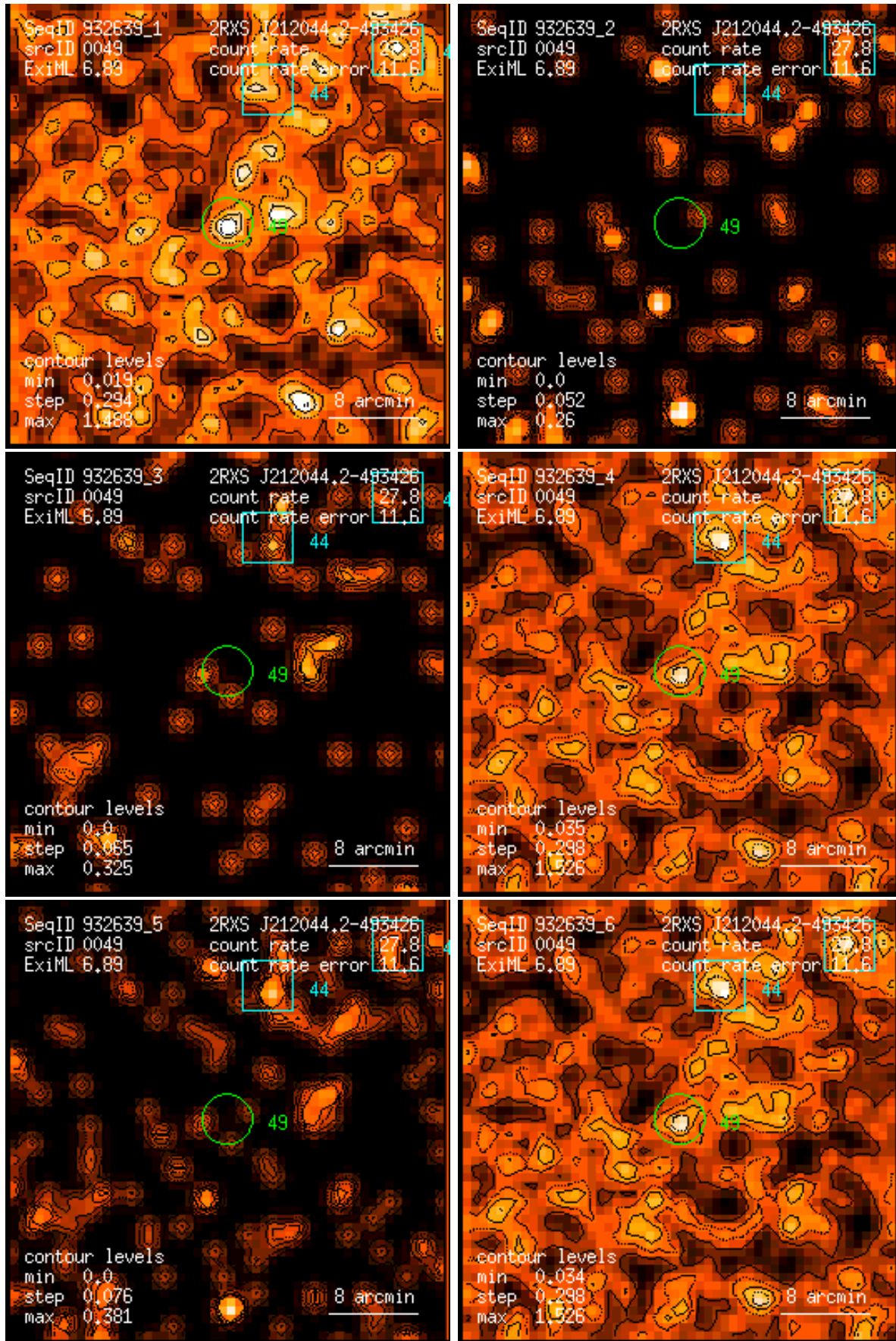
Figure 49: RASS 932639: detection 0049: band rate images, Gaussian filter: (1) PSPC channels 11 – 41, (2) 52 – 90, (3) 91 – 201, (4) 11 – 235, (5) 52 – 201, (6) 11 – 201. Broad band rates in counts/ks. Band rate contour levels in counts/ks/arcmin 2 .
