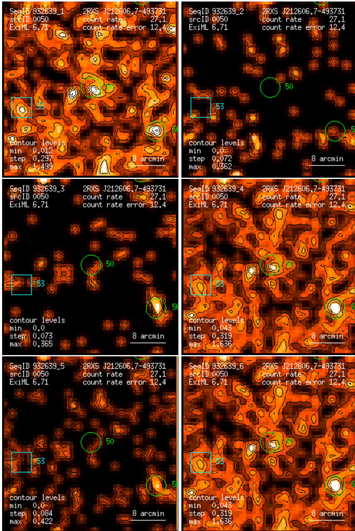
Figure 50: RASS 932639: detection 0050: band rate images, Gaussian filter: (1) PSPC channels 11 – 41, (2) 52 – 90, (3) 91 – 201, (4) 11 – 235, (5) 52 – 201, (6) 11 – 201. Broad band rates in counts/ks. Band rate contour levels in counts/ks/arcmin 2 .
