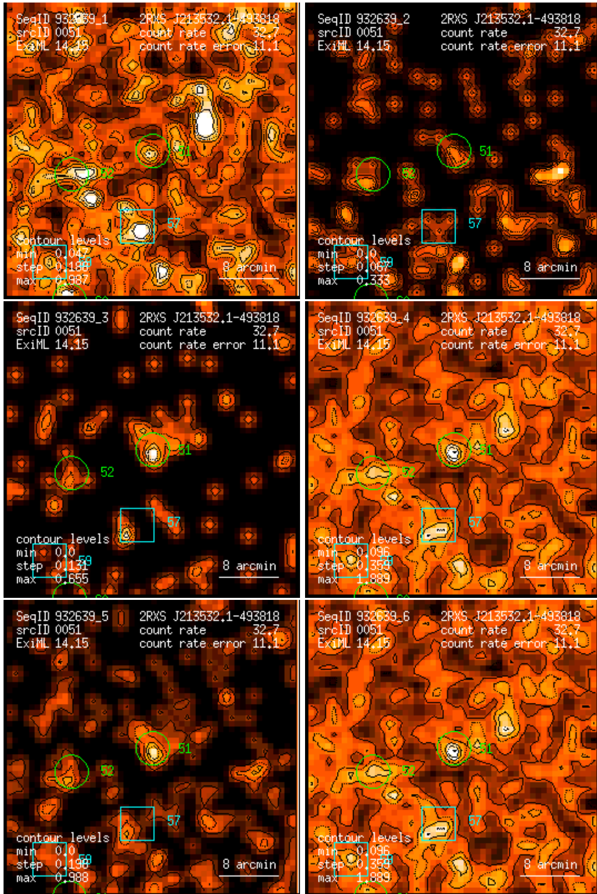
Figure 51: RASS 932639: detection 0051: band rate images, Gaussian filter: (1) PSPC channels 11 – 41, (2) 52 – 90, (3) 91 – 201, (4) 11 – 235, (5) 52 – 201, (6) 11 – 201. Broad band rates in counts/ks. Band rate contour levels in counts/ks/arcmin 2 .
