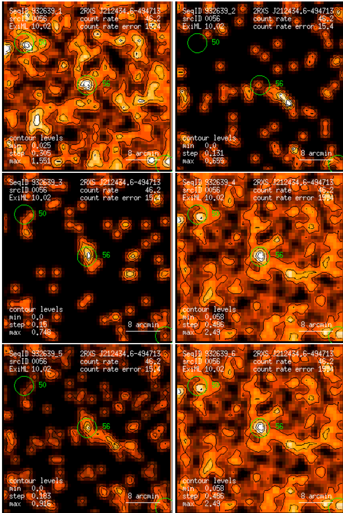
Figure 56: RASS 932639: detection 0056: band rate images, Gaussian filter: (1) PSPC channels 11 – 41, (2) 52 – 90, (3) 91 – 201, (4) 11 – 235, (5) 52 – 201, (6) 11 – 201. Broad band rates in counts/ks. Band rate contour levels in counts/ks/arcmin 2 .
