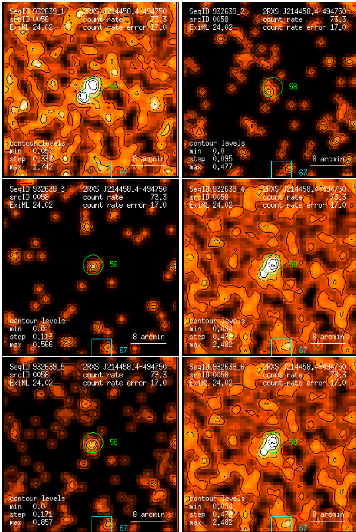
Figure 58: RASS 932639: detection 0058: band rate images, Gaussian filter: (1) PSPC channels 11 – 41, (2) 52 – 90, (3) 91 – 201, (4) 11 – 235, (5) 52 – 201, (6) 11 – 201. Broad band rates in counts/ks. Band rate contour levels in counts/ks/arcmin 2 .
