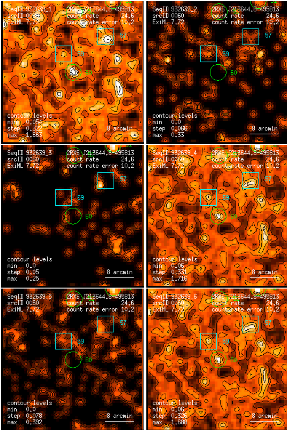
Figure 60: RASS 932639: detection 0060: band rate images, Gaussian filter: (1) PSPC channels 11 – 41, (2) 52 – 90, (3) 91 – 201, (4) 11 – 235, (5) 52 – 201, (6) 11 – 201. Broad band rates in counts/ks. Band rate contour levels in counts/ks/arcmin 2 .
