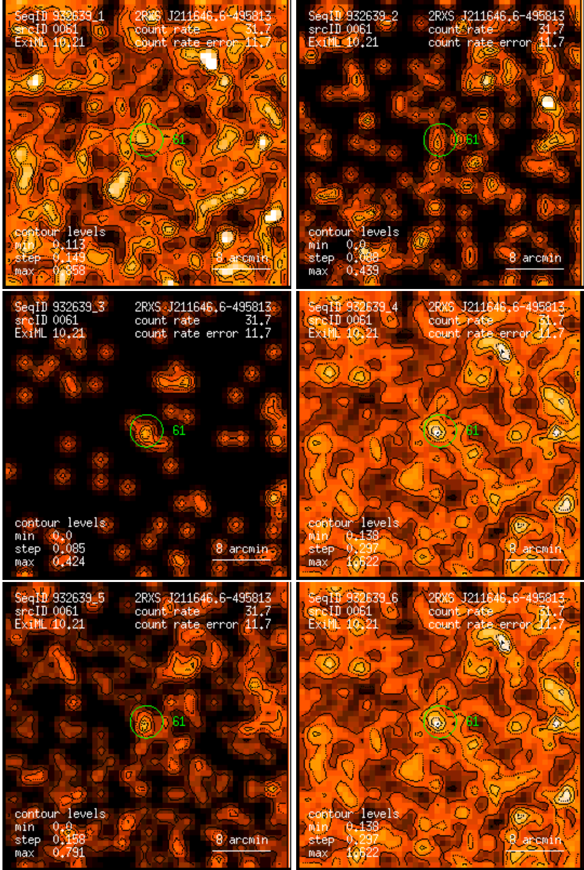
Figure 61: RASS 932639: detection 0061: band rate images, Gaussian filter: (1) PSPC channels 11 – 41, (2) 52 – 90, (3) 91 – 201, (4) 11 – 235, (5) 52 – 201, (6) 11 – 201. Broad band rates in counts/ks. Band rate contour levels in counts/ks/arcmin 2 .
