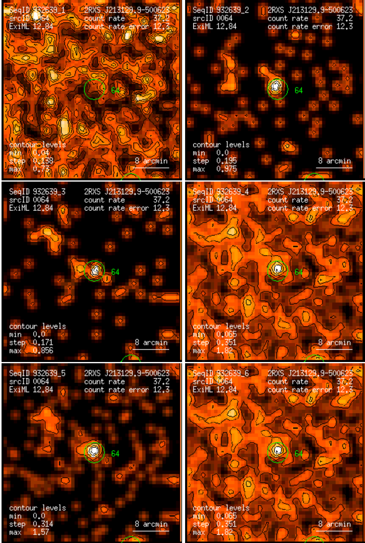
Figure 64: RASS 932639: detection 0064: band rate images, Gaussian filter: (1) PSPC channels 11 – 41, (2) 52 – 90, (3) 91 – 201, (4) 11 – 235, (5) 52 – 201, (6) 11 – 201. Broad band rates in counts/ks. Band rate contour levels in counts/ks/arcmin 2 .
