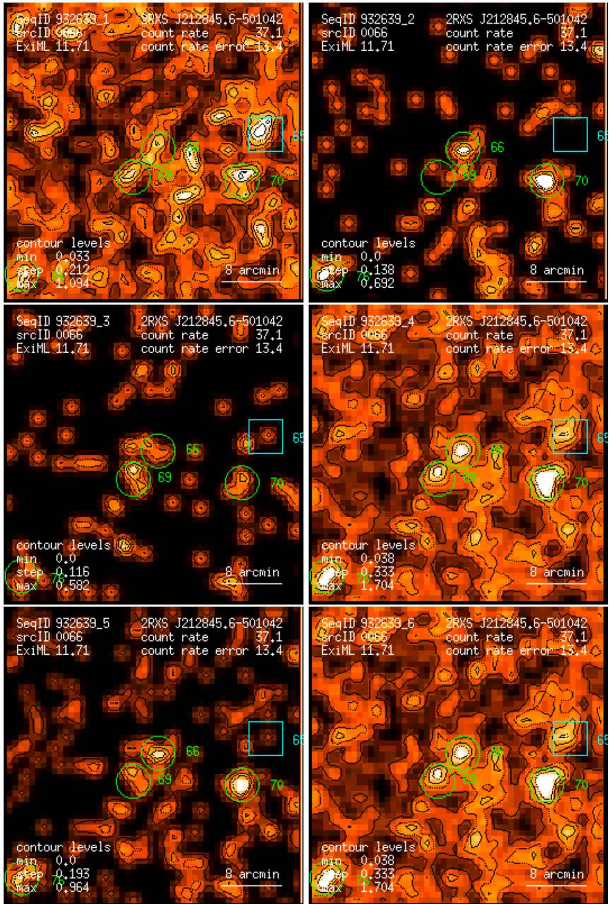
Figure 66: RASS 932639: detection 0066: band rate images, Gaussian filter: (1) PSPC channels 11 – 41, (2) 52 – 90, (3) 91 – 201, (4) 11 – 235, (5) 52 – 201, (6) 11 – 201. Broad band rates in counts/ks. Band rate contour levels in counts/ks/arcmin 2 .
