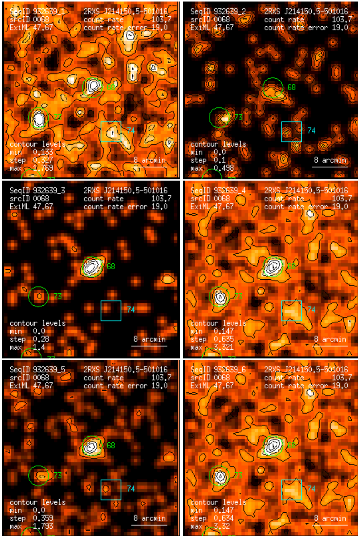
Figure 68: RASS 932639: detection 0068: band rate images, Gaussian filter: (1) PSPC channels 11 – 41, (2) 52 – 90, (3) 91 – 201, (4) 11 – 235, (5) 52 – 201, (6) 11 – 201. Broad band rates in counts/ks. Band rate contour levels in counts/ks/arcmin 2 .
