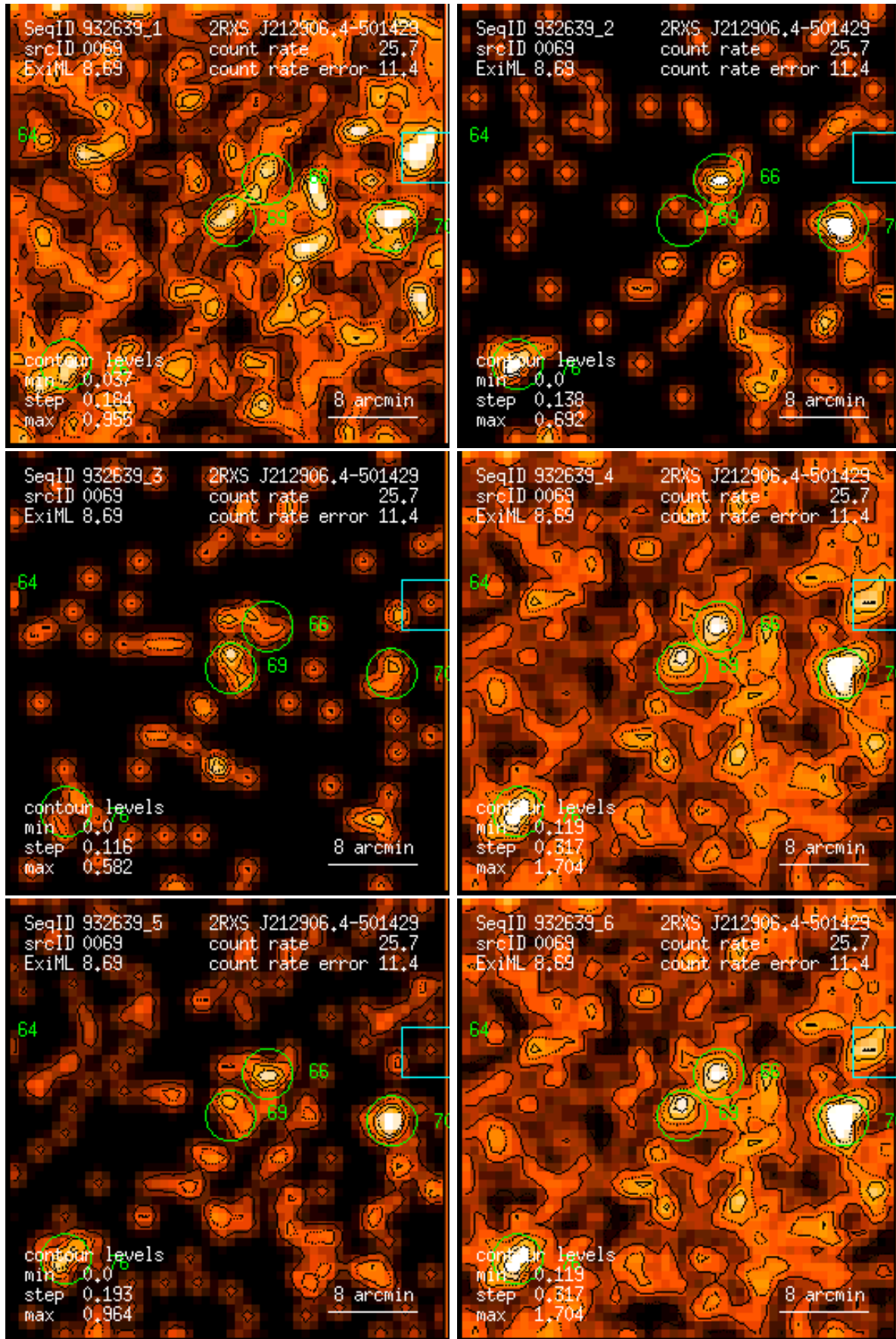
Figure 69: RASS 932639: detection 0069: band rate images, Gaussian filter: (1) PSPC channels 11 – 41, (2) 52 – 90, (3) 91 – 201, (4) 11 – 235, (5) 52 – 201, (6) 11 – 201. Broad band rates in counts/ks. Band rate contour levels in counts/ks/arcmin 2 .
