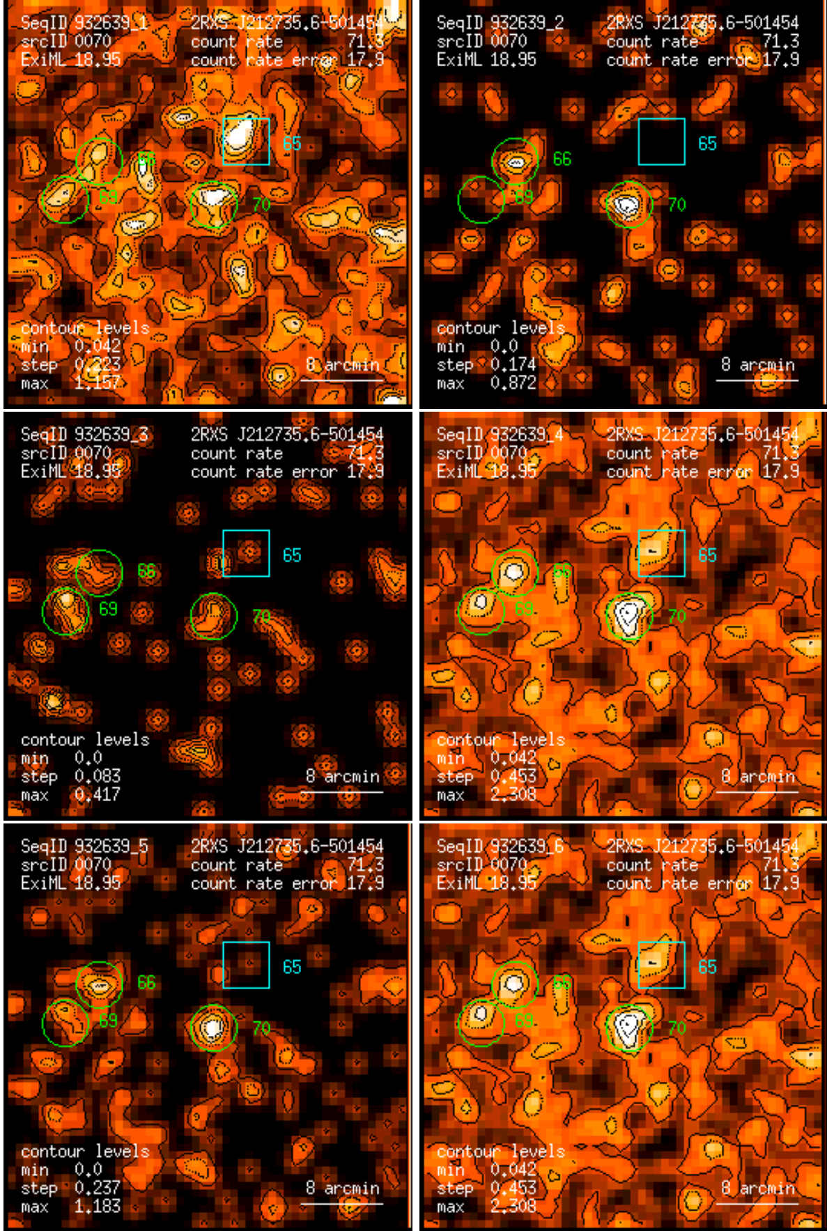
Figure 70: RASS 932639: detection 0070: band rate images, Gaussian filter: (1) PSPC channels 11 – 41, (2) 52 – 90, (3) 91 – 201, (4) 11 – 235, (5) 52 – 201, (6) 11 – 201. Broad band rates in counts/ks. Band rate contour levels in counts/ks/arcmin 2 .
